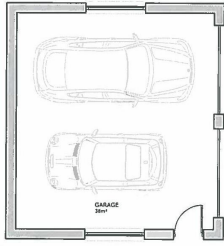
01 PROPOSED GARAGE PLAN 1:100
